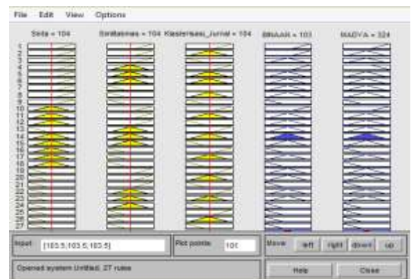
Fig 5. Defuzzification Calculation Process
